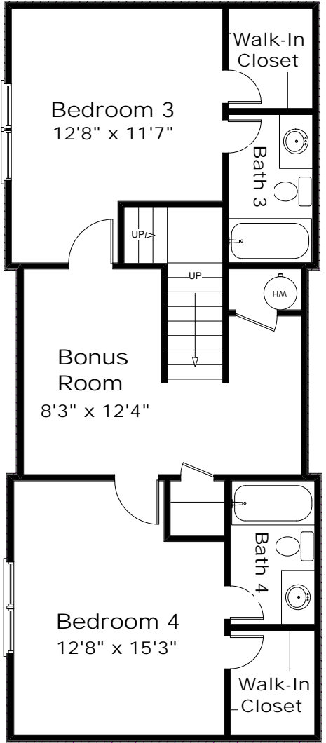
3rd Floor 821 SF
