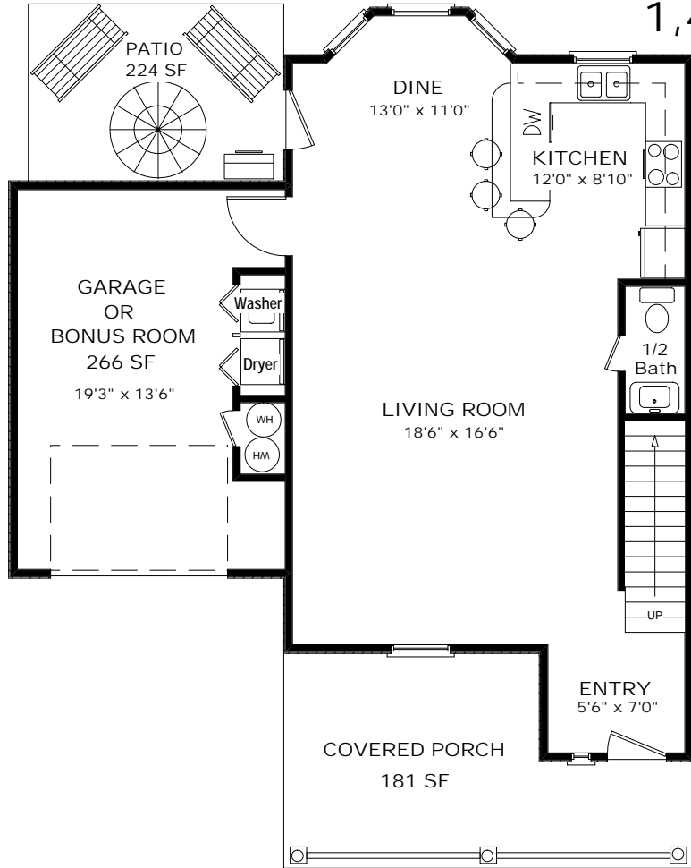
Downstairs Floor Plan
